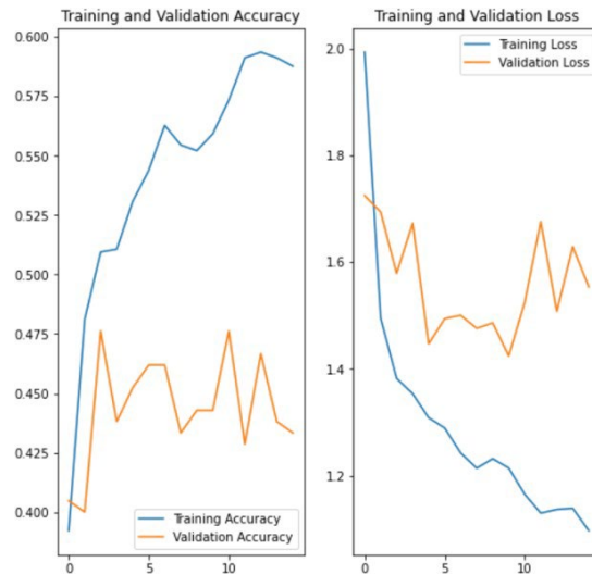
Figure 5. Graphs of Training and Validation Accuracy and Loss.
