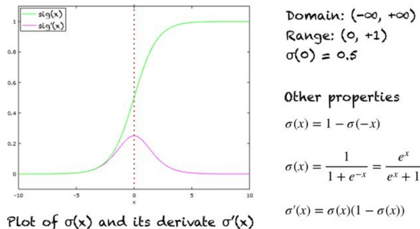
Figure 2. Logistic Sigmoid Function [7].
