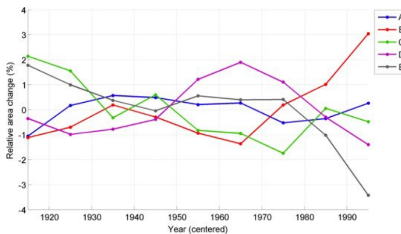
Figure 1. Area change of major Koeppen types [2].
