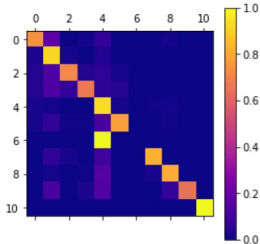
Figure 7. Confusion Matrix with Climate Types.
